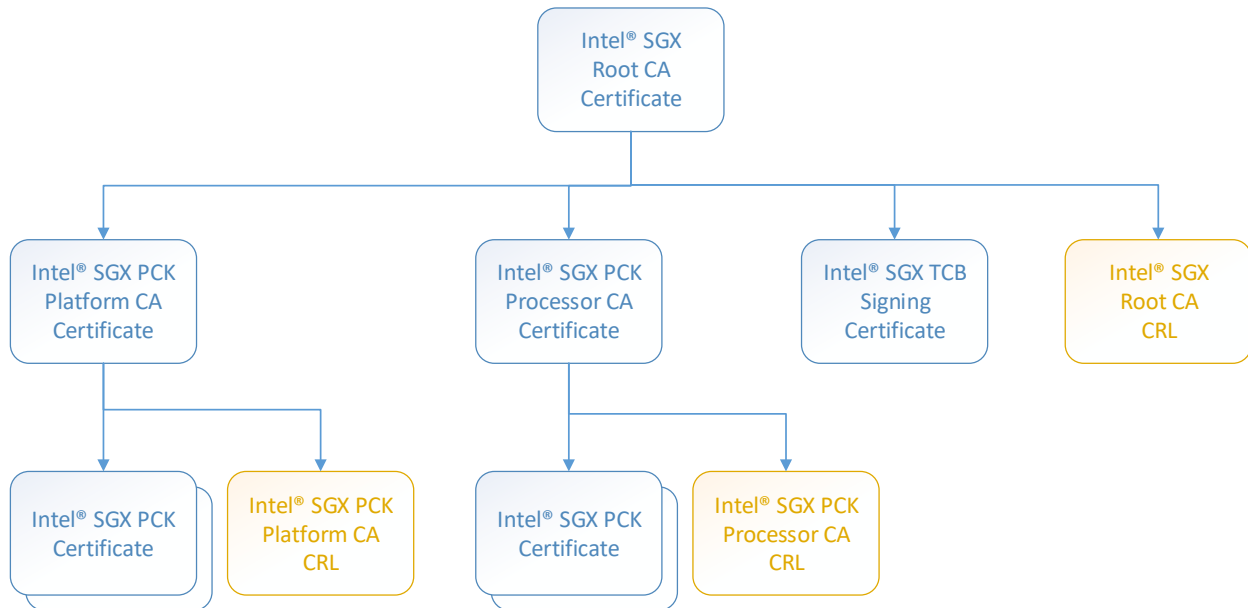
Figure 2-1: Certificate Hierarchy
