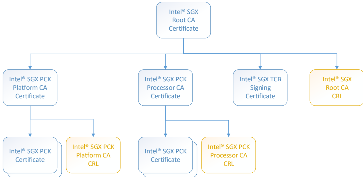
Figure 0-1: Certificate Hierarchy
