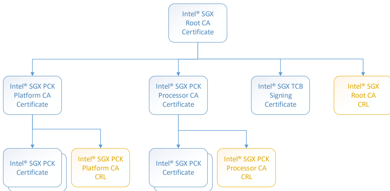
Figure 2-1: Certificate Hierarchy
