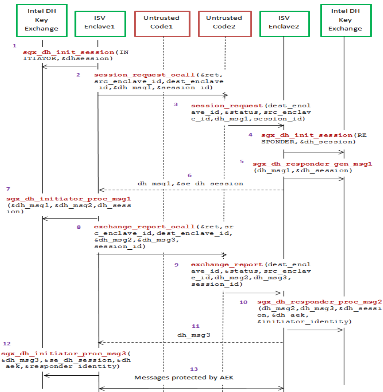
Figure 5 Local Attestation Flow with the DH Key Exchange Library
